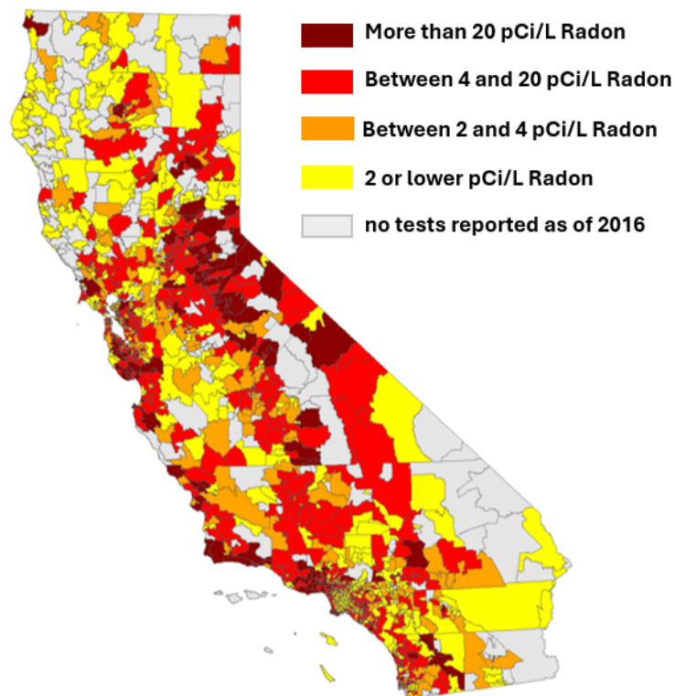
Figure 1: Maximum Reported Indoor Radon Level By Zip Code
